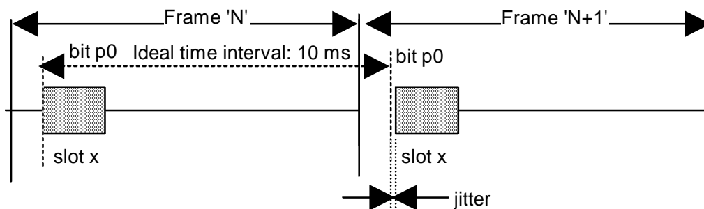
Figure 29: Jitter definition
