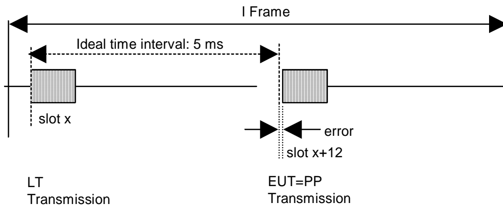
Figure 30: PP packet transmission error definition
