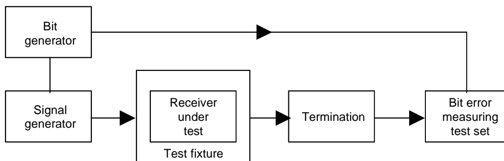
Figure B.2: Measurement arrangement No.2
