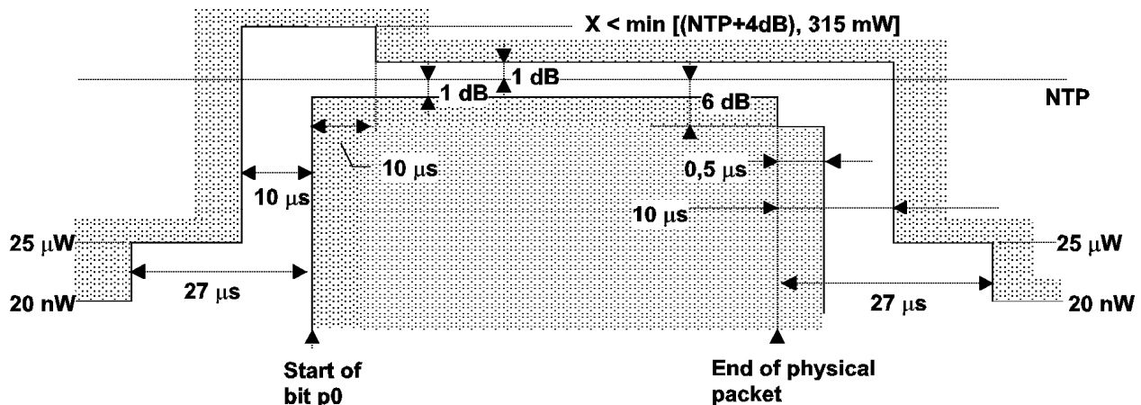
Figure 31: Power-time template
