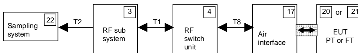
Figure 15: Test setup 1
