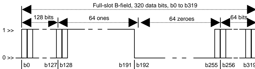
Figure 34: Test packet transmission for case 2, full-slot
