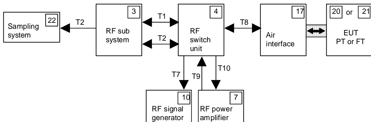
Figure 19: Test setup 5
