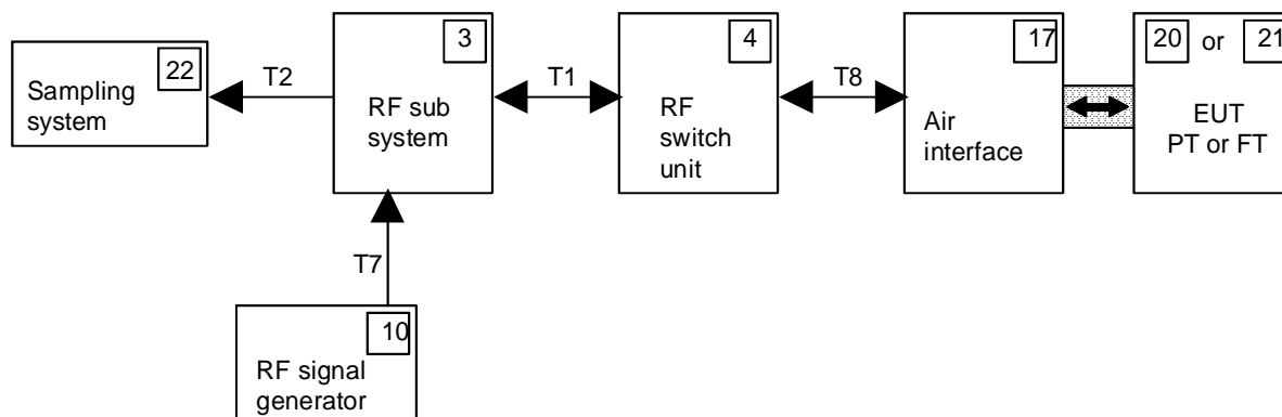
Figure 16: Test setup 2
