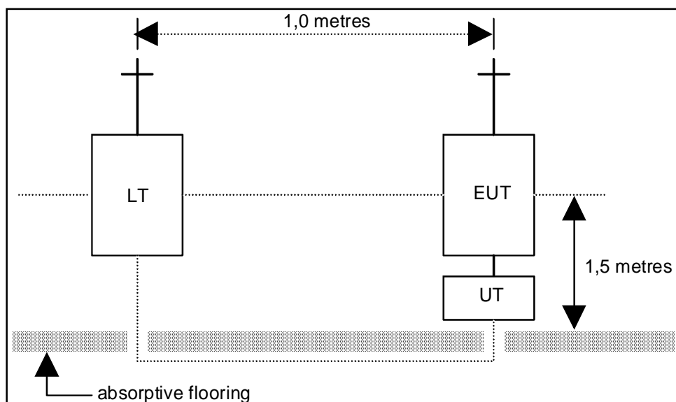
Figure 21: Testing arrangement
