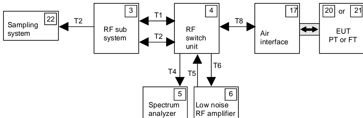
Figure 18: Test setup 4
