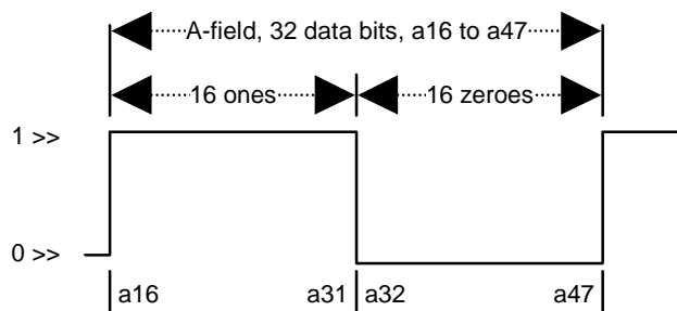
Figure 32: Test packet structure for case 2, A-field
