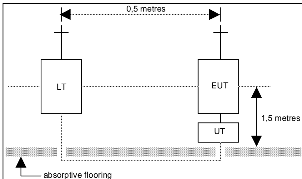
Figure 20: Testing arrangement
