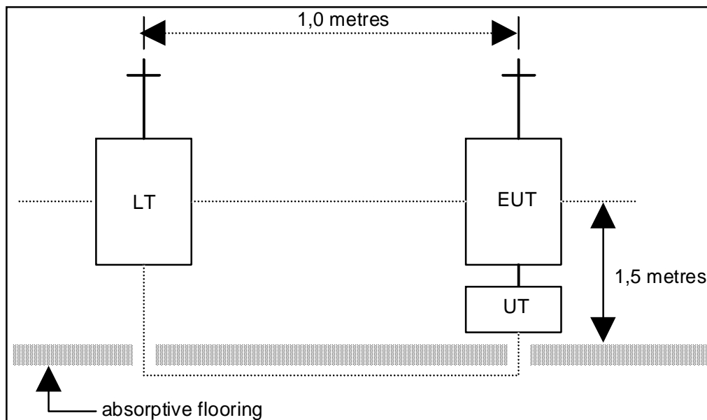
Figure 22: Testing arrangement
